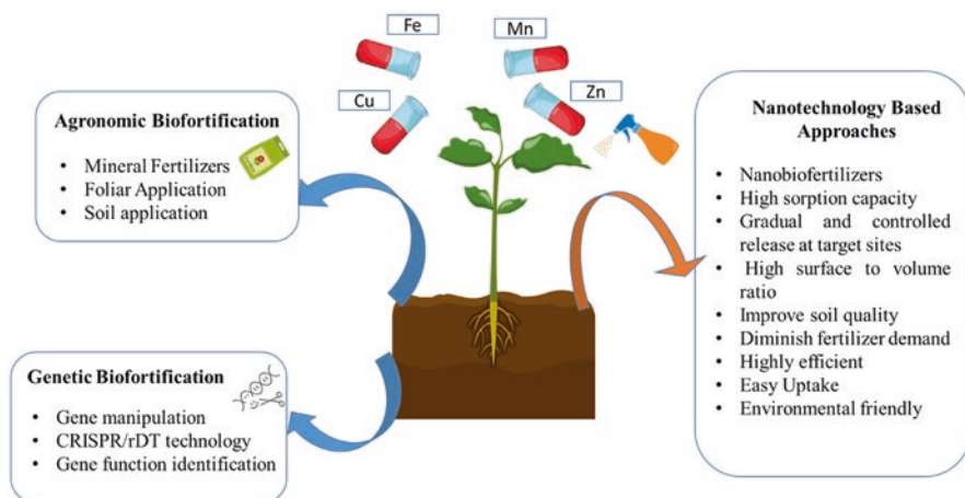
Fig. 2.1 Biofortification approaches
